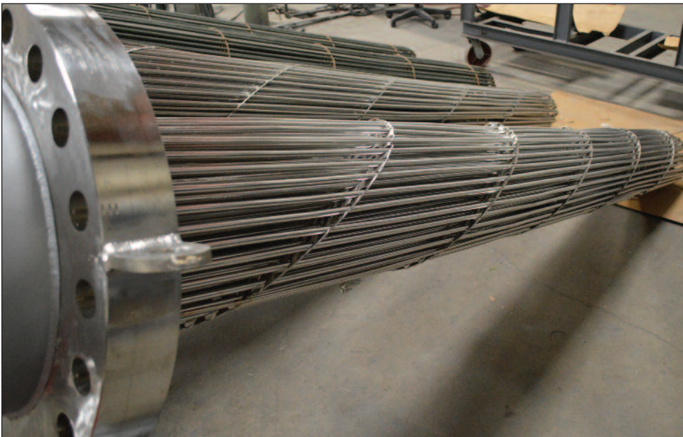
Angled turbulators - optimum heat transfer
